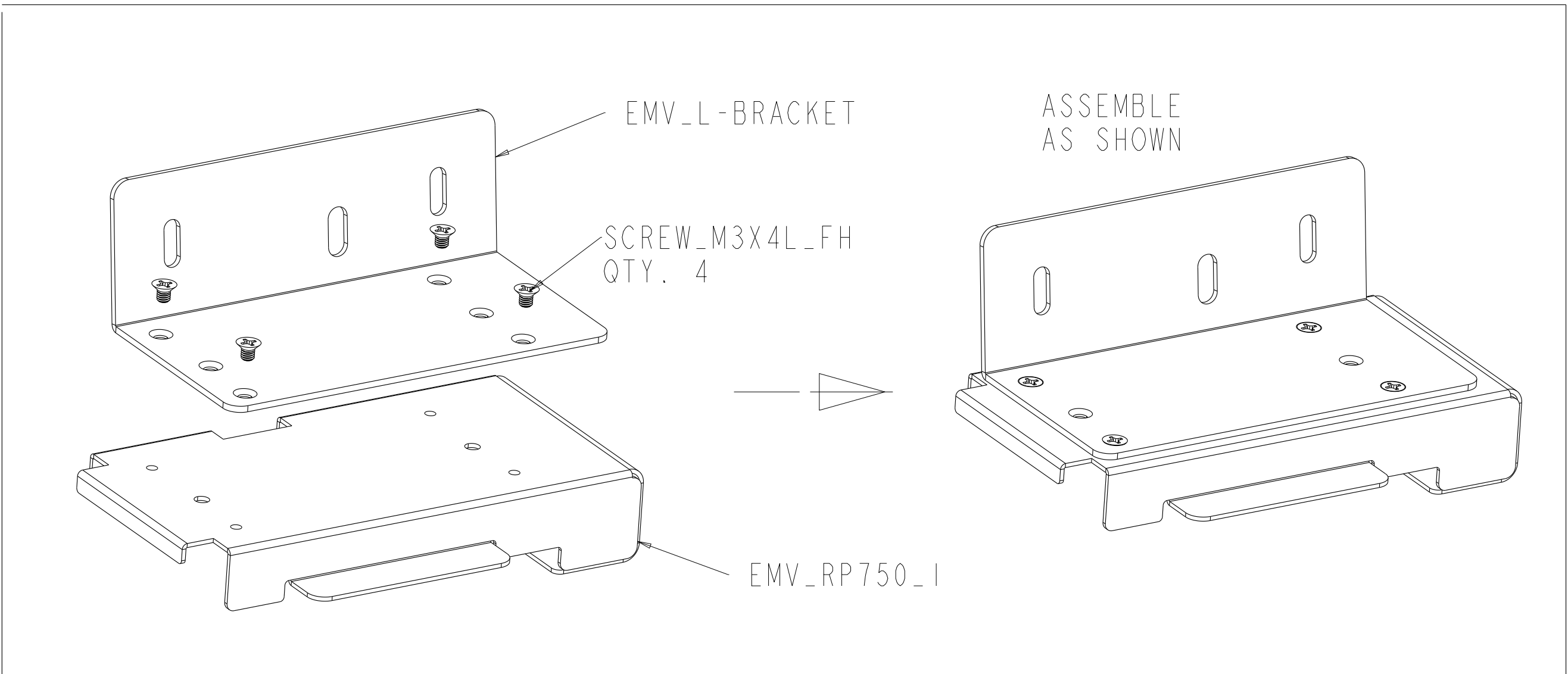
EMV_RP750_1.ASM QTY. PER KIT
